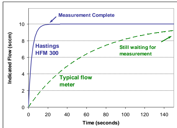
Figure 3 Comparison of Hastings HFM 300 to Typical Flow Meter Times
